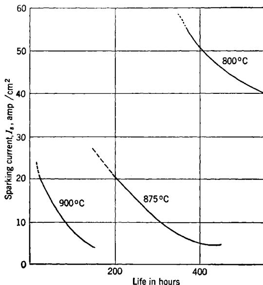
FIG. 12-5.—The expected life, at three different temperatures, of a double-carbonate coating on Grade A nickel. Test conditions: 1 \mu sec; 400 PRF; 10 amp/cm 2 .
